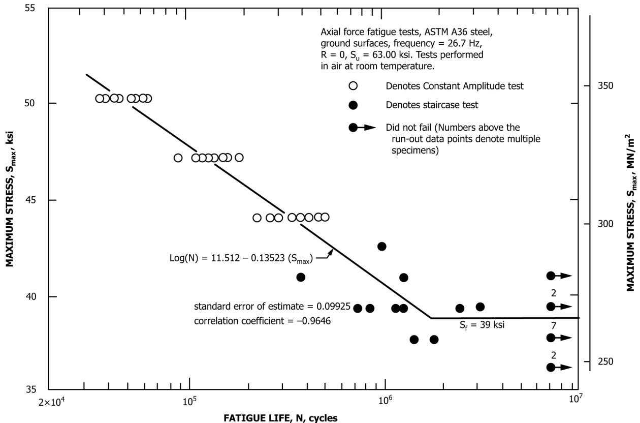
FIG. 1 S-N Diagram (historic)
